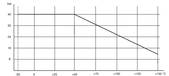
diagramma pressione/temperatura pressure/temperature diagram
