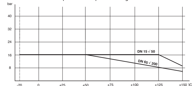
diagramma pressione/temperatura pressure/temperature diagram
